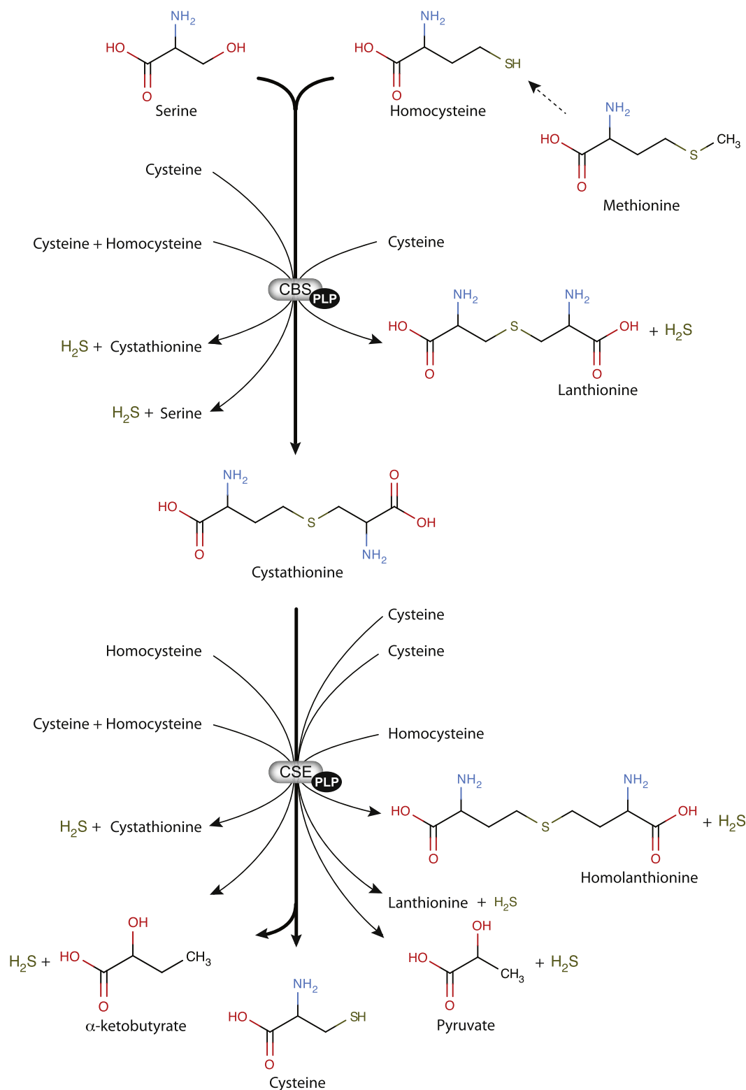
Fig. 4. The transsulfuration pathway, H 2 S production and the enzymes involved. Methionine is activated to the universal methyl donor, S-adenosylmethionine, which is converted to S-adenosylhomocysteine during S-adenosylmethionine-dependent transmethylation reactions. S-adenosylhomocysteine in turn is hydrolyzed to adenosine and homocysteine in a reaction catalyzed by S-adenosylhomocysteine hydrolase (not shown). Homocysteine is either remethylated to methionine (not shown) or converted to cysteine via the transsulfuration pathway, where homocysteine is converted to cysteine through the sequential action of two PLP-dependent enzymes, cystathionine β-synthase (CBS; EC 4.2.1.22) and cystathionine γ-lyase (CSE; EC 4.4.1.1). H 2 S is produced through seven non-canonical reactions catalyzed by CBS and CSE, as indicated.
